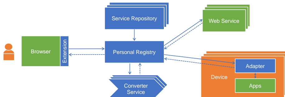
Fig. 1. Linking services to websites: Architecture of Semantic Data Mediator
